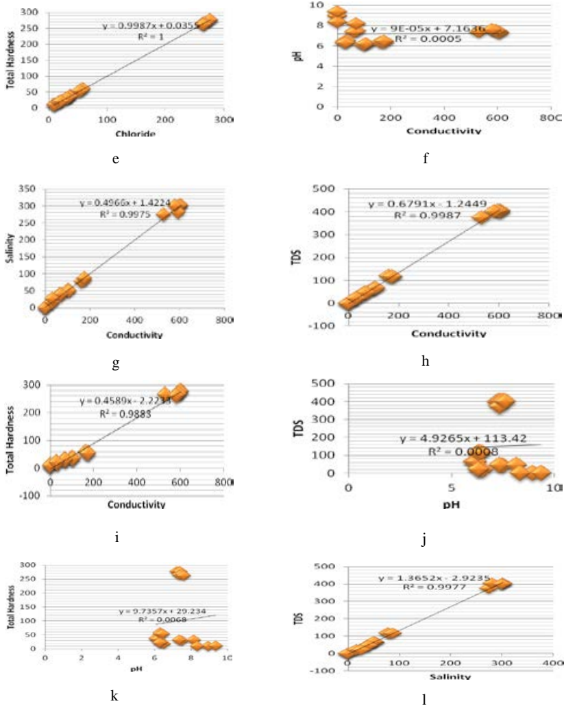
Figure 3. (a) Scatter plot of (a) chloride and conductivity (b) chloride and pH (c) chloride and salinity (d) chloride and TDS (e) chloride and total hardness (f) conductivity and pH (g) conductivity and salinity (h) conductivity and TDS (i) conductivity and total hardness (j) pH
