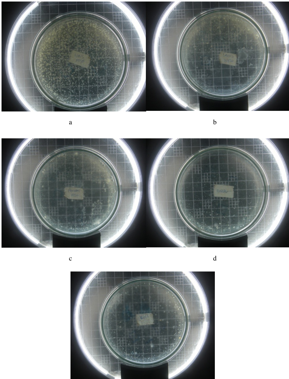
Figure 4. Heterotrophic Plate Count (HPC) of (a) libis well, (b) lawis well, (c) Pandan well, (d) Kinalagi spring, (e) rainwater from a private tank.
